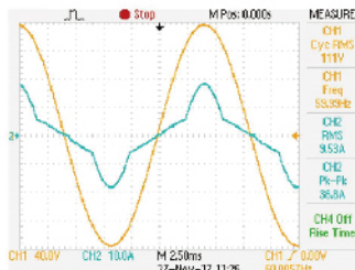
110V, 5A + 22ohm Test Waveform 110V, 10A + 11ohm Test Waveform PV Inverter 测试的Non-Linear CC+CR mode(CC+CR)
